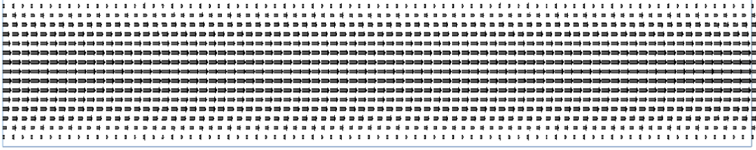
Fig. 2. Central cross-section of flow through the first test problem using the new formulation of the Navier-Stokes equations with \alpha = 10 and \mathbf{n} \cdot \mathbf{r} = \mathbf{n} \cdot \left(\frac{1}{\sqrt{Re}} \nabla \times \omega\right) along all boundaries.
