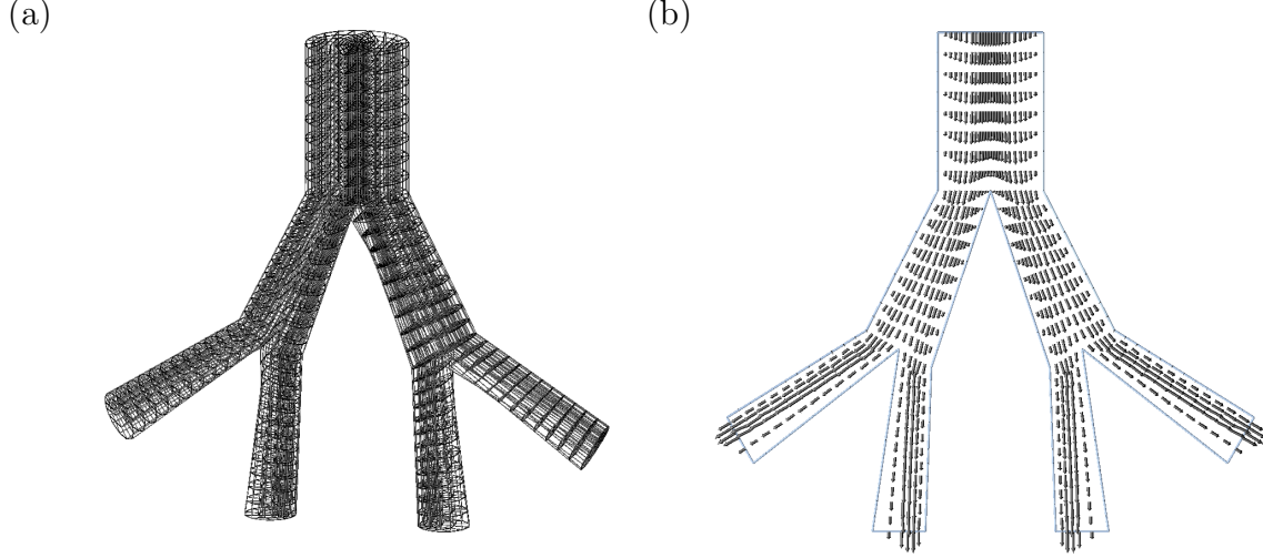
Fig. 4. (a) The finite element mesh for the third test problem composed of 420 hexahedral elements.(b) Velocity vectors for the central cross-section using a triquadratic basis and \alpha = 10 .
