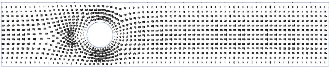
Fig. 3. (a) A cross-section of the finite element mesh for the second test problem. The domain is 5 \times 1 \times 1 and the cylindrical obstruction has a diameter of 0.4. (b) Velocity vectors for the central cross-section using a triquadratic basis and \alpha = 10 .
