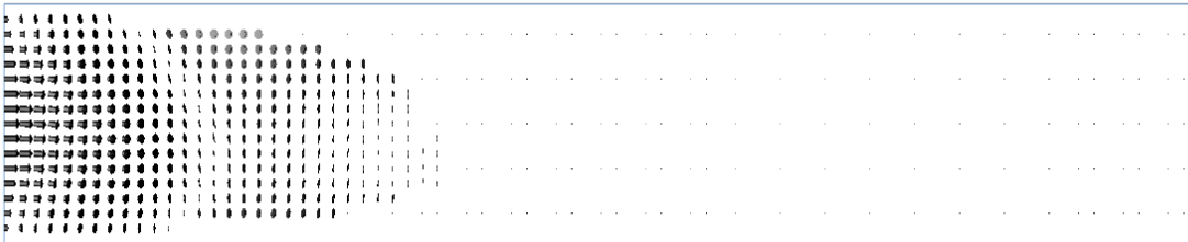
Fig. 1. Central cross-section of flow through the first test problem using the standard vorticity formulation of the Navier-Stokes equations.
